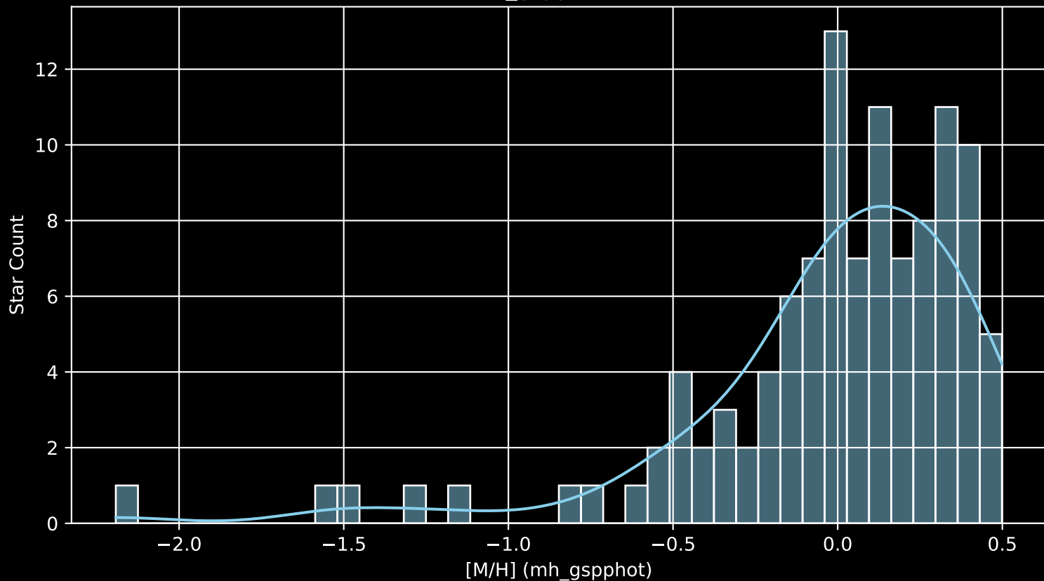
APOGEE DR17 Field: [SMC5 [M/H] (mh_gspphot) (n= 110)
