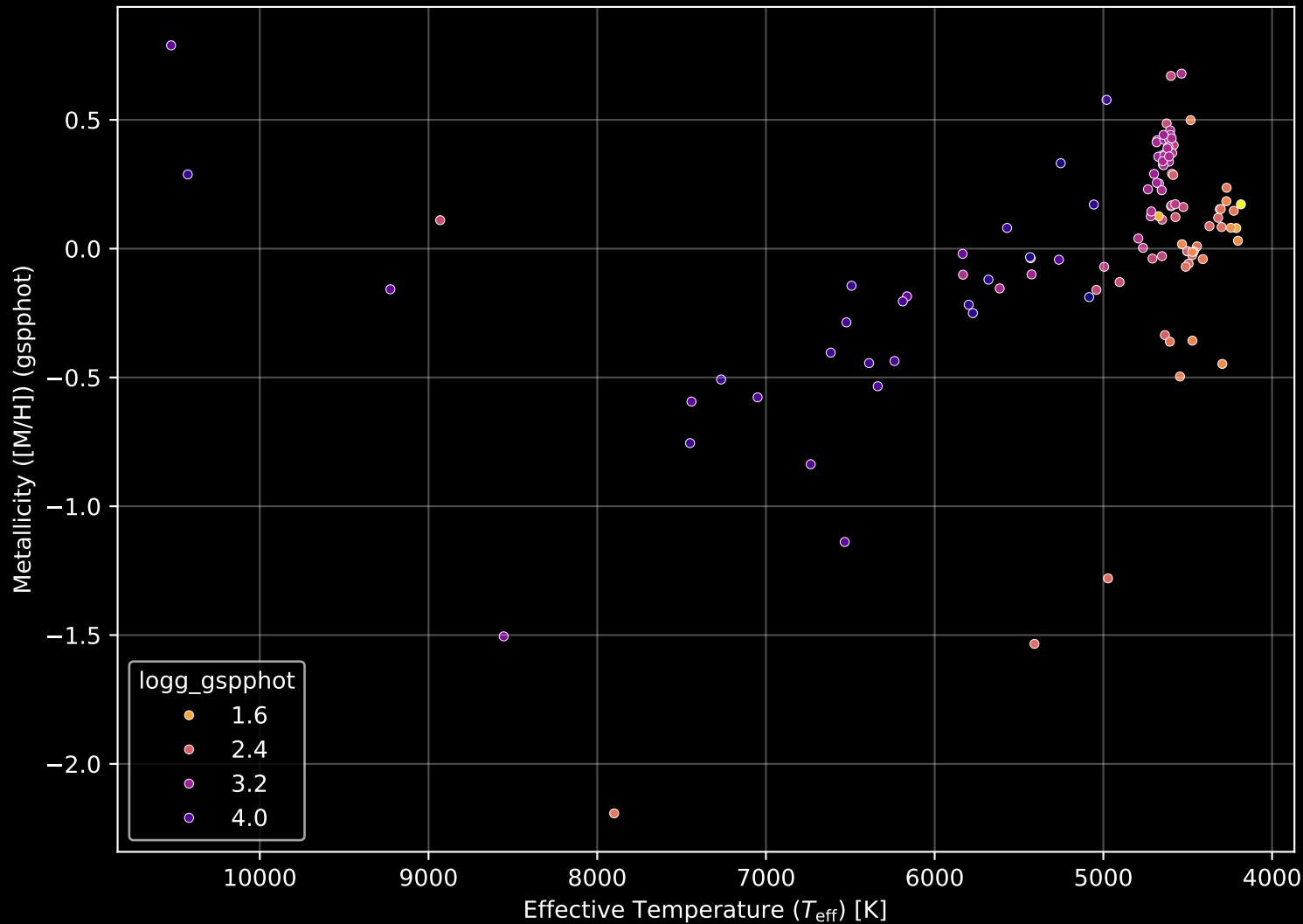
APOGEE DR17 Field: [SMC5] Stellar Population Parameters (n= 114)
