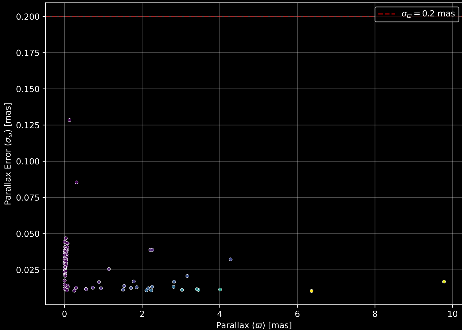
APOGEE DR17 Field: [SMC5] Parallax Quality (n= 114)
