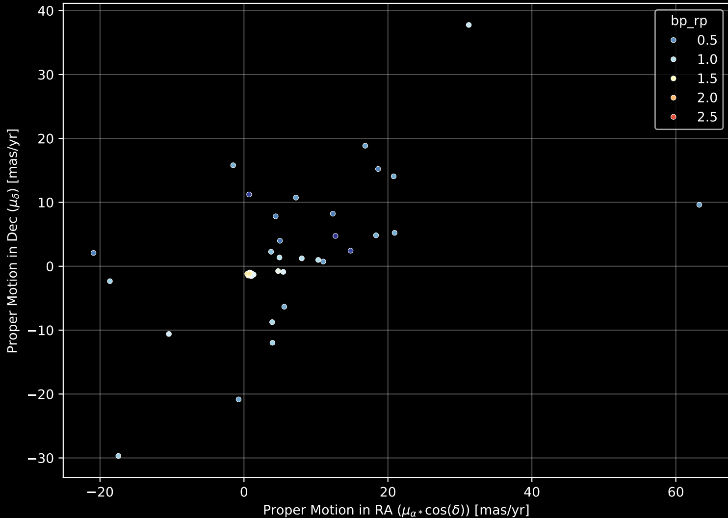
APOGEE DR17 Field: [SMC5] Proper Motion Diagram (n= 114)
