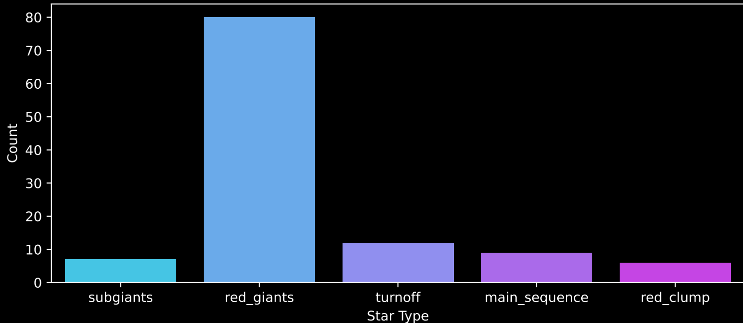
APOGEE DR17 Field: [SMC5] Count plot of Star Type
