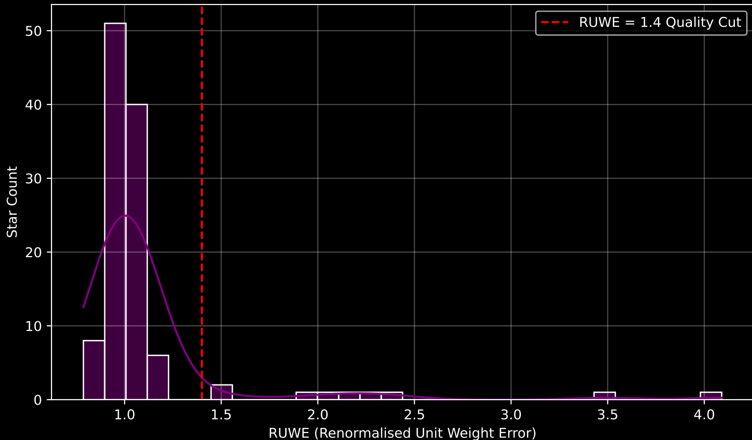
GAPOGEE DR17 Field [SMC5] RUWE Distribution (n= 114)
